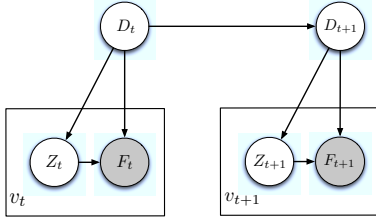
Figure 5. Graphical model of the non-negative hidden Markov model.
