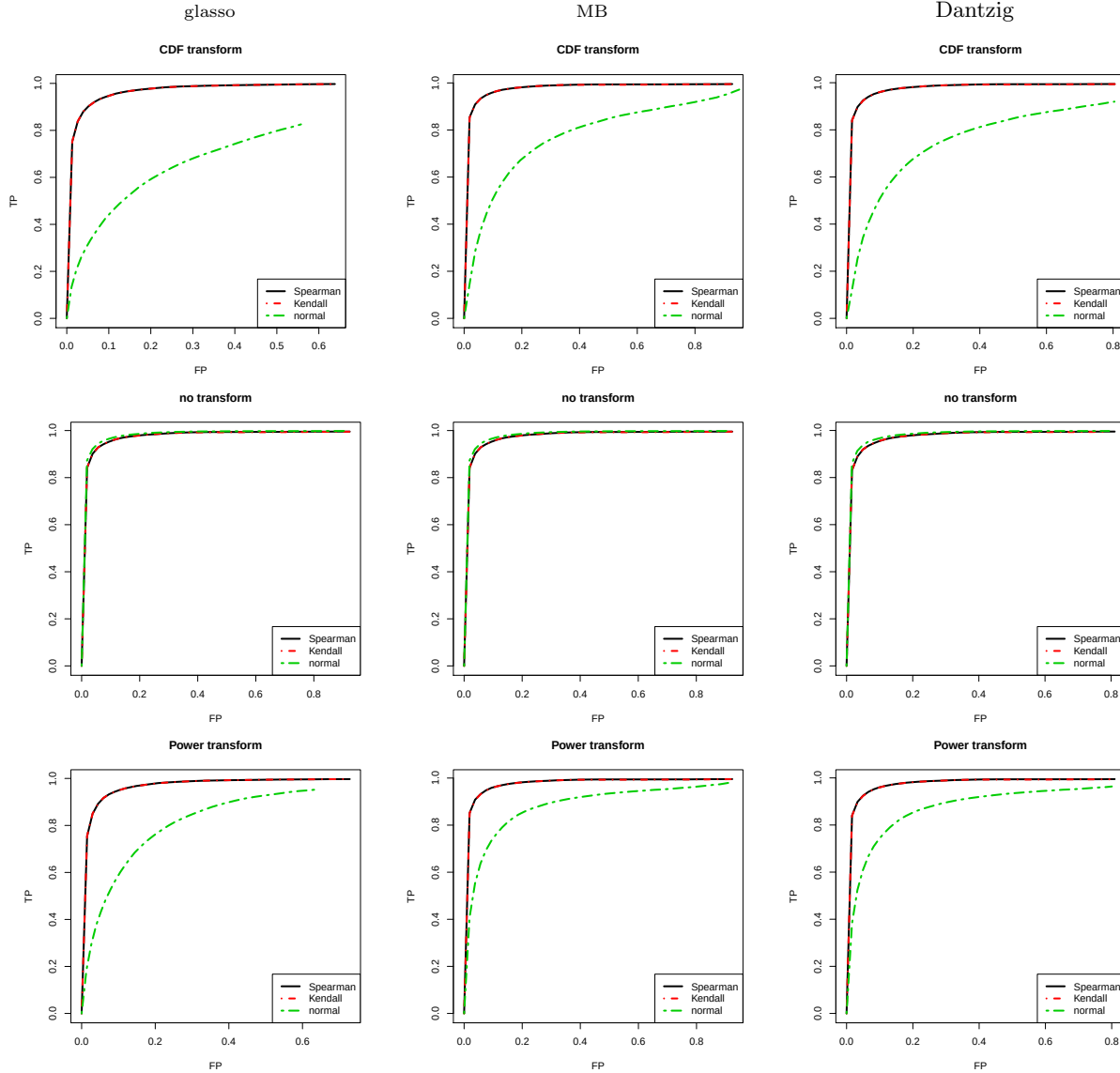
Figure 1. ROC curves for the cdf, linear (or no transformation) and power transformations (top, middle, bottom) using the glasso, parallel lasso and graphical Dantzig selector. Here n = 200 and d = 100 .
