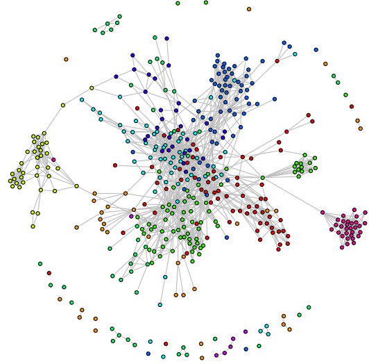
Figure 2. The nonparanormal SKEPTIC graph estimated from the S&P 500 stock data from Jan. 1, 2003 to Jan. 1, 2008. Nodes are colored according to their GICS sectors.
