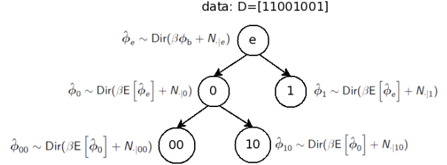
Figure 1. An example Dirichlet-VMM tree for a binary sequence. Contexts 01 and 11 are only observed once and thus are not included in the tree. Note that for readability, contexts in this figure are denoted in chronological order.
