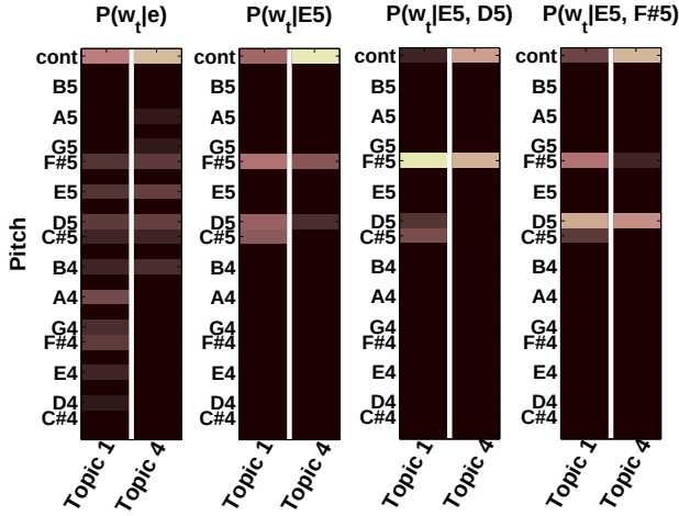
Figure 7. Conditional distributions over notes for 2 topics that are mostly assigned in pieces from the key of D . Each distribution is conditioned on a different context. Model: Variable-gram.De.T 50 .
