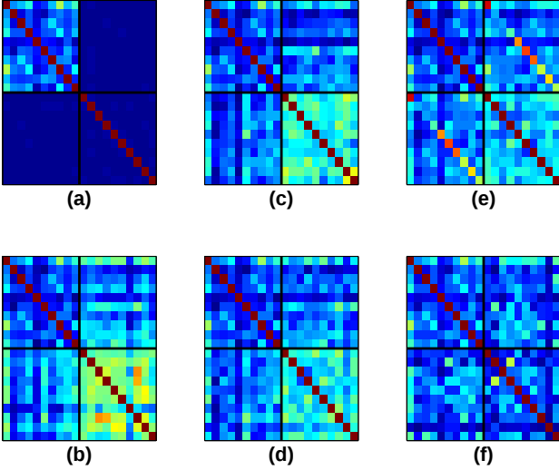
Figure 5. (4, 1) mismatch kernels computed between 10 test sequences (rows 1-10) and 10 model samples (rows 11-20). (a) Uniform(26) (b) Dirichlet-VMM.De (c) Topic Bigram.50 (d) Topic Var-gram.De.50 (e) Topic Var-gram.De.50-Given topics (f) Traindata
