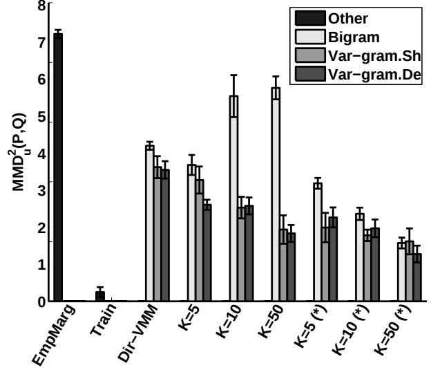
Figure 4. Estimated squared MMD between test sequences and model samples using the (4, 1) mismatch kernel. Colour describes the temporal structure in a model. Groups describe models with different numbers of topics. EmpMarg: the empirical marginal distribution of the training data. Train: the train sequences. (*): The models are sampled conditional on the topic allocations (see text for details).
